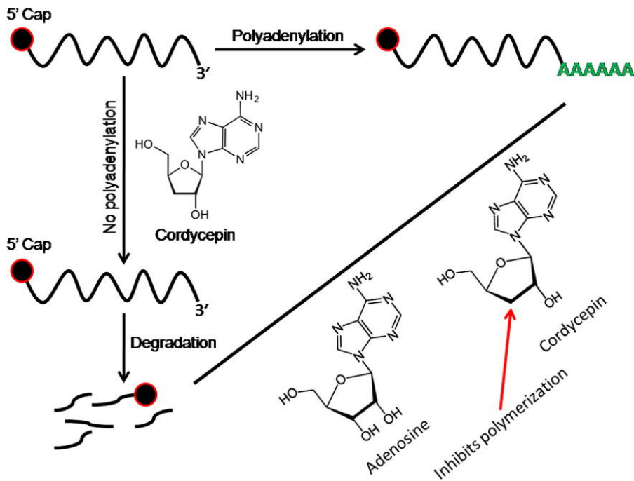
Figure 4. Cordycepin mediated biological response for SARS-CoV-2 RNA degradation.
