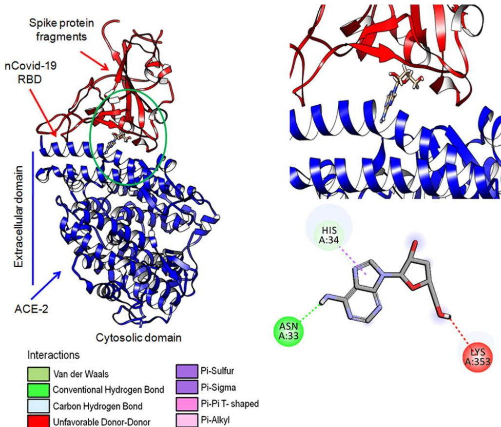
Figure 1. Docking structure and chemical interactions of cordycepin have been shown along with ligand atoms and interacting amino acids in the binding sites of the SARS-CoV-2 spike protein RBD.
