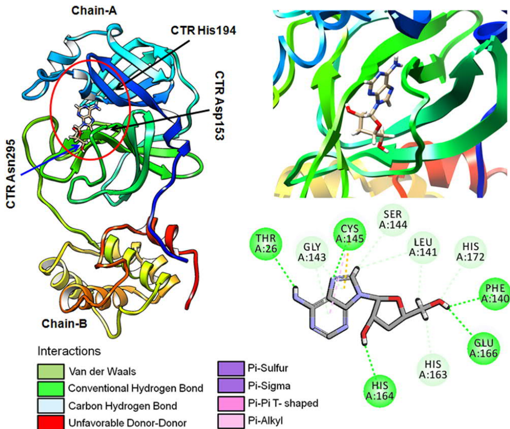
Figure 2. Docking structure and chemical interactions of cordycepin have been shown along with ligand atoms and interacting amino acids in the binding sites of M pro .
