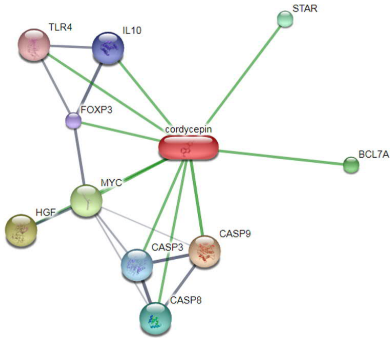
Figure 3. The interaction network of cordycepin was determined by STITCH algorithm, showing the involvement of cordycepin in multiple pathways. This is the confidence view; stronger associations are represented by thicker lines. Protein-protein interactions are shown in grey, chemical-protein interactions in green and interactions between chemicals in red.
